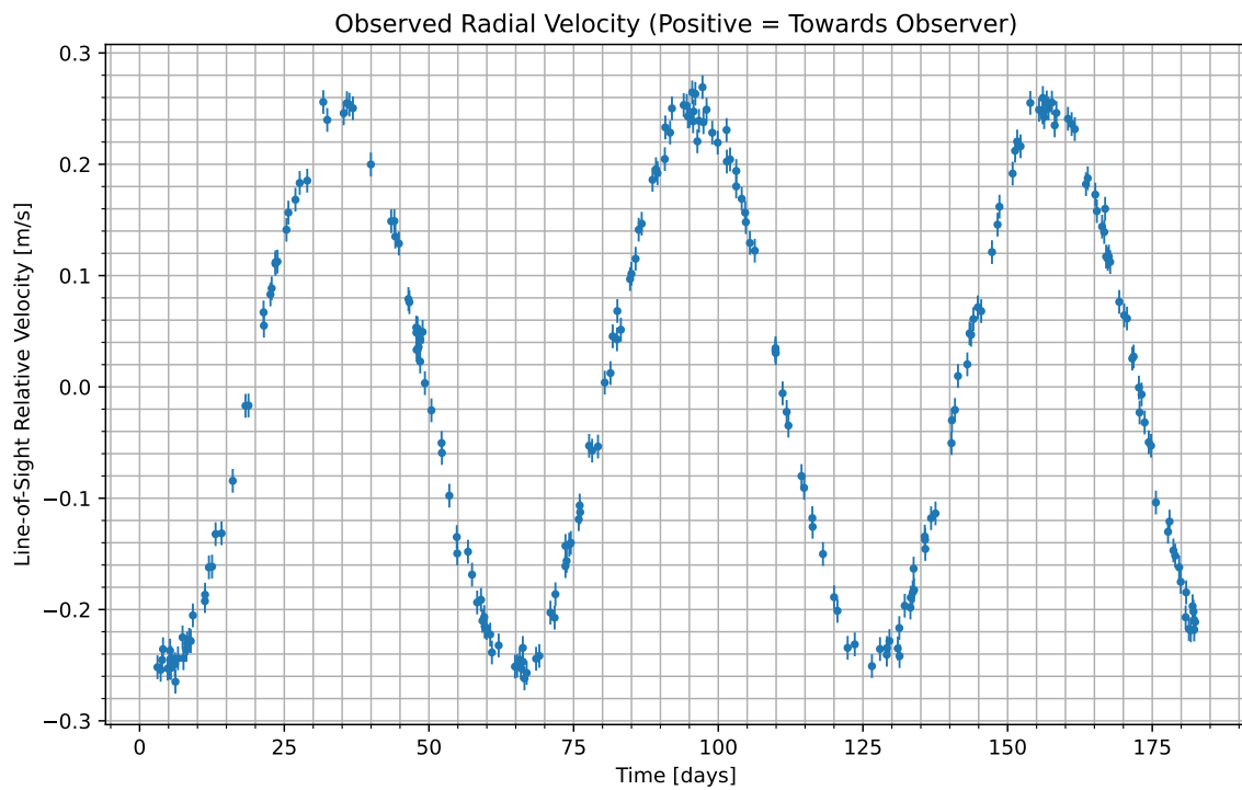
Figure 1: We have isolated the radial velocity of the host star due to the candidate planet. Data begins at UTC 2079-03-07/23:47. Positive values indicate the velocity at which the star is moving towards us; negative indicate the velocity at which it is moving away.
