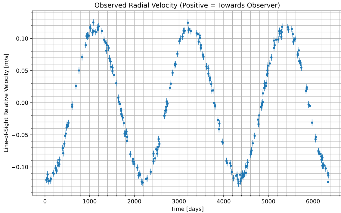
Figure 1: We have isolated the radial velocity of the host star due to the candidate planet. Data begins at UTC 2078-07-22/20:58. Positive values indicate the velocity at which the star is moving towards us; negative indicate the velocity at which it is moving away.
