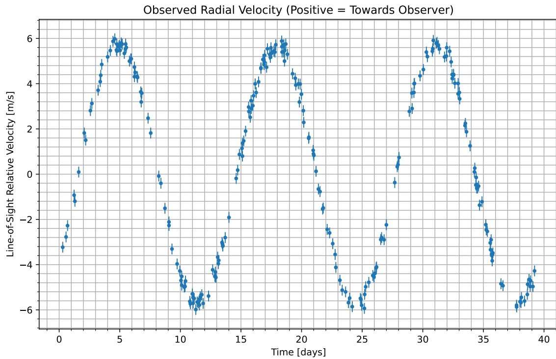
Figure 1: We have isolated the radial velocity of the host star due to the candidate planet. Data begins at UTC 2074-07-25/20:01. Positive values indicate the velocity at which the star is moving towards us; negative indicate the velocity at which it is moving away.
