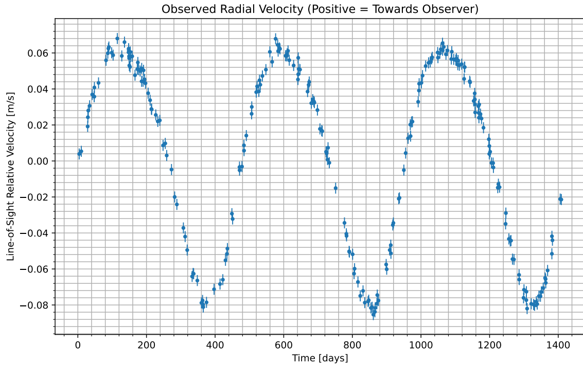
Figure 1: We have isolated the radial velocity of the host star due to the candidate planet. Data begins at UTC 2068-01-06/01:31. Positive values indicate the velocity at which the star is moving towards us; negative indicate the velocity at which it is moving away.
