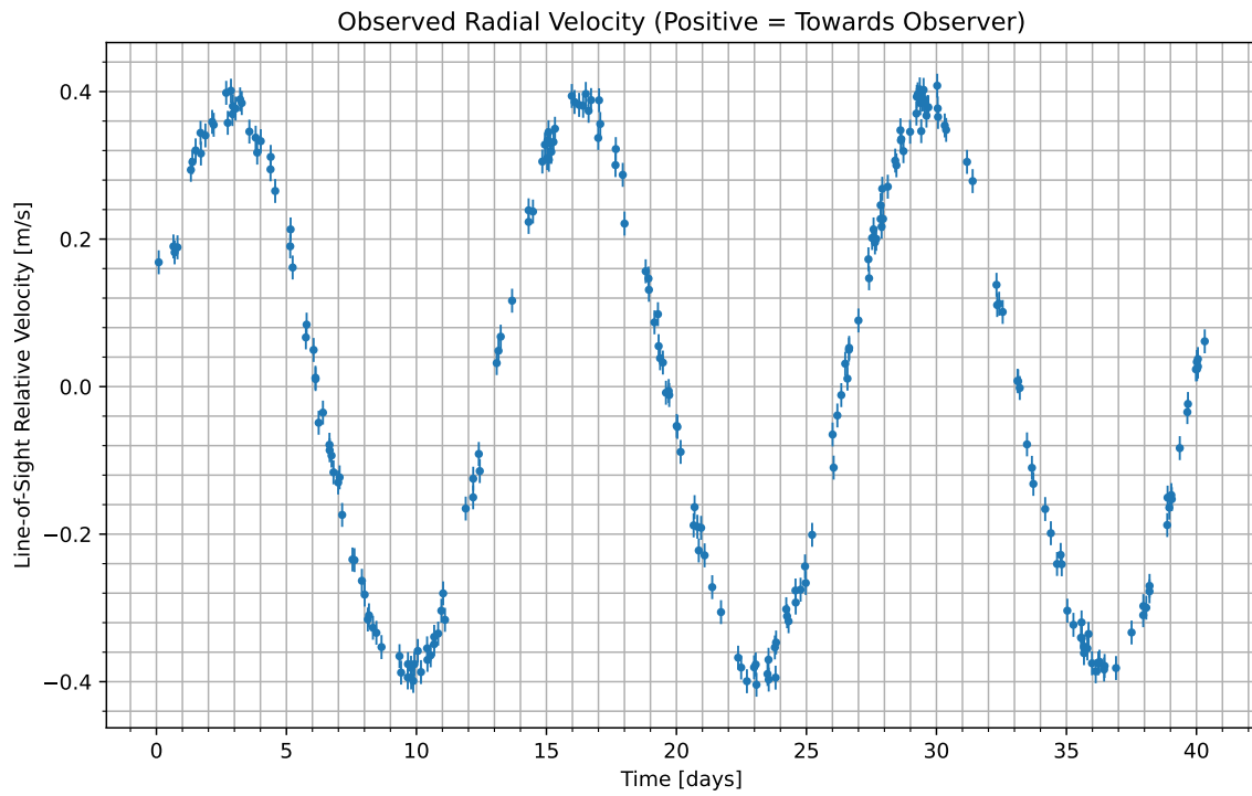
Figure 1: We have isolated the radial velocity of the host star due to the candidate planet. Data begins at UTC 2096-11-18/02:02. Positive values indicate the velocity at which the star is moving towards us; negative indicate the velocity at which it is moving away.
