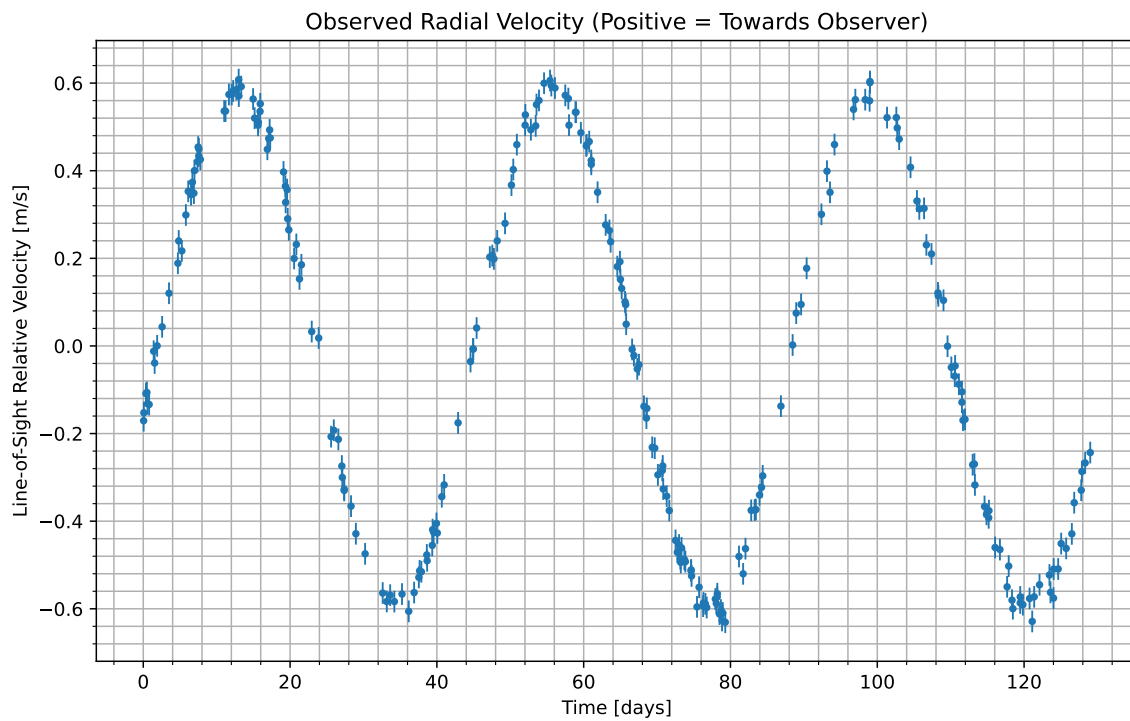
Figure 1: We have isolated the radial velocity of the host star due to the candidate planet. Data begins at UTC 2100-01-15/04:00. Positive values indicate the velocity at which the star is moving towards us; negative indicate the velocity at which it is moving away.
