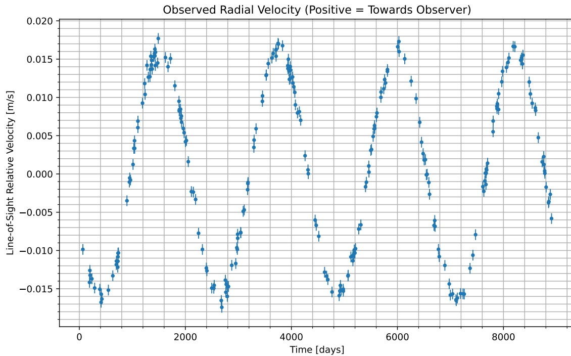
Figure 1: We have isolated the radial velocity of the host star due to the candidate planet. Data begins at UTC 2063-07-11/07:33. Positive values indicate the velocity at which the star is moving towards us; negative indicate the velocity at which it is moving away.
