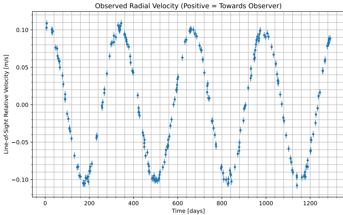
Figure 1: We have isolated the radial velocity of the host star due to the candidate planet. Data begins at UTC 2094-11-07/18:14. Positive values indicate the velocity at which the star is moving towards us; negative indicate the velocity at which it is moving away.
