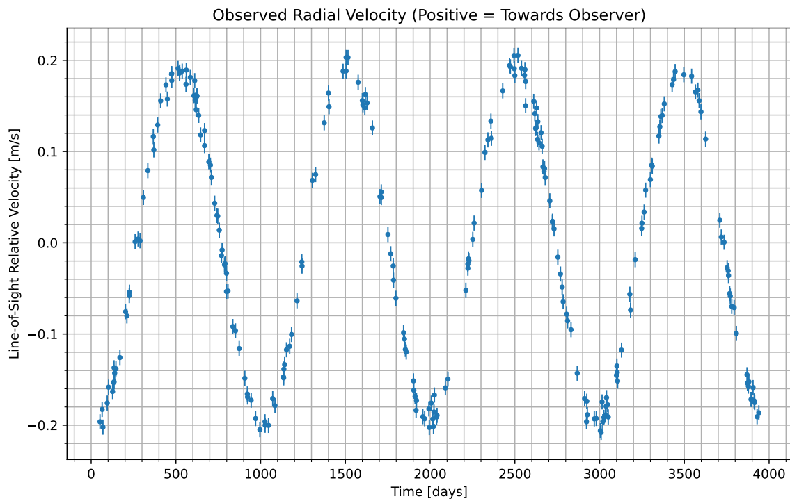
Figure 1: We have isolated the radial velocity of the host star due to the candidate planet. Data begins at UTC 2066-10-12/13:20. Positive values indicate the velocity at which the star is moving towards us; negative indicate the velocity at which it is moving away.
