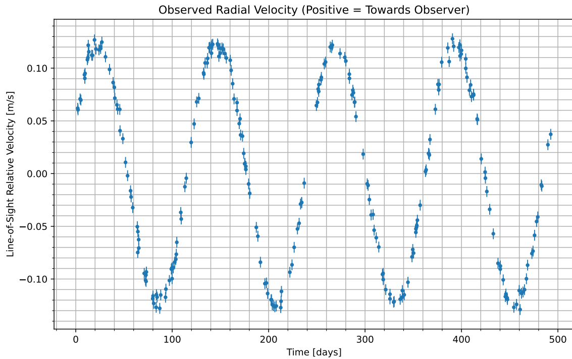
Figure 1: We have isolated the radial velocity of the host star due to the candidate planet. Data begins at UTC 2091-07-06/14:38. Positive values indicate the velocity at which the star is moving towards us; negative indicate the velocity at which it is moving away.
