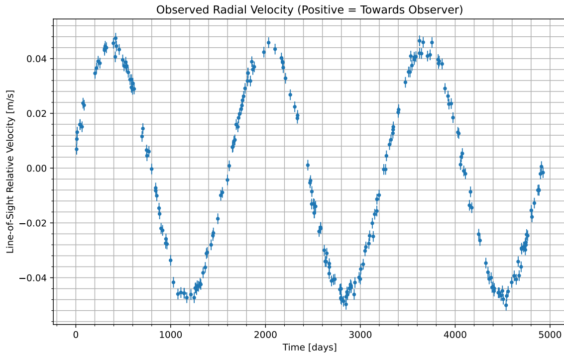
Figure 1: We have isolated the radial velocity of the host star due to the candidate planet. Data begins at UTC 2071-05-09/16:01. Positive values indicate the velocity at which the star is moving towards us; negative indicate the velocity at which it is moving away.
