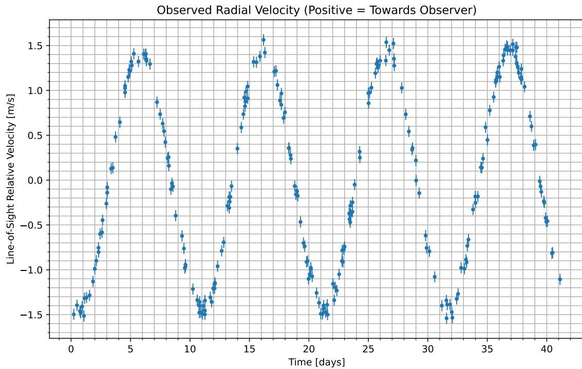
Figure 1: We have isolated the radial velocity of the host star due to the candidate planet. Data begins at UTC 2087-10-31/18:54. Positive values indicate the velocity at which the star is moving towards us; negative indicate the velocity at which it is moving away.
