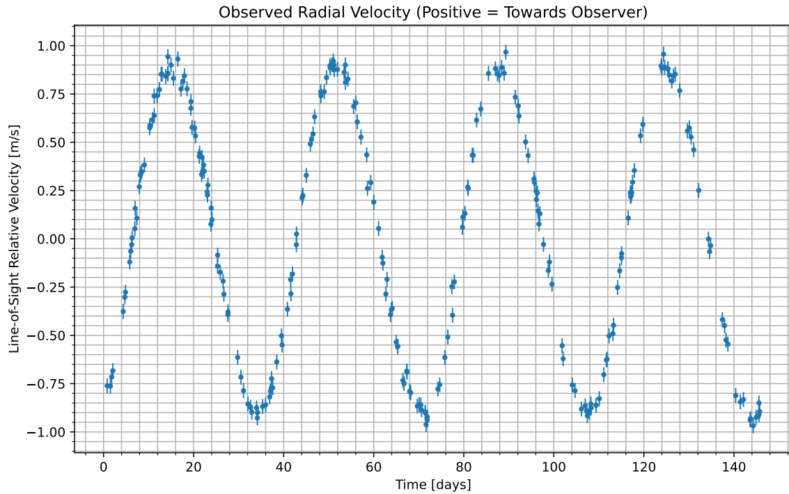
Figure 1: We have isolated the radial velocity of the host star due to the candidate planet. Data begins at UTC 2095-04-15/16:32. Positive values indicate the velocity at which the star is moving towards us; negative indicate the velocity at which it is moving away.
