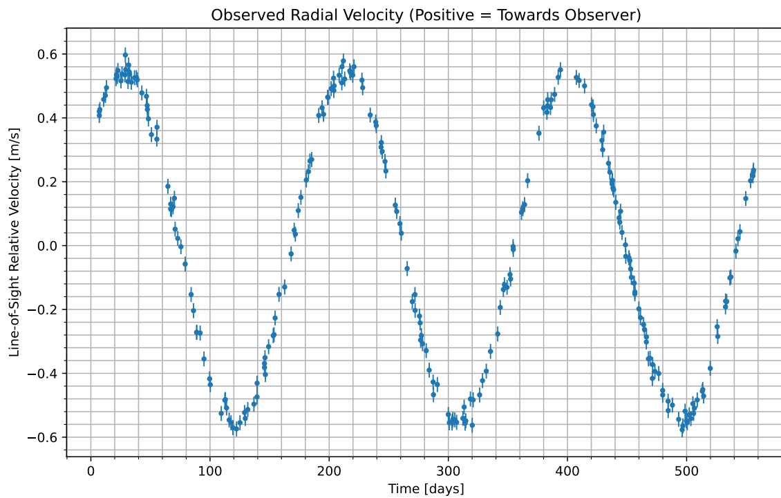
Figure 1: We have isolated the radial velocity of the host star due to the candidate planet. Data begins at UTC 2095-03-14/05:17. Positive values indicate the velocity at which the star is moving towards us; negative indicate the velocity at which it is moving away.
