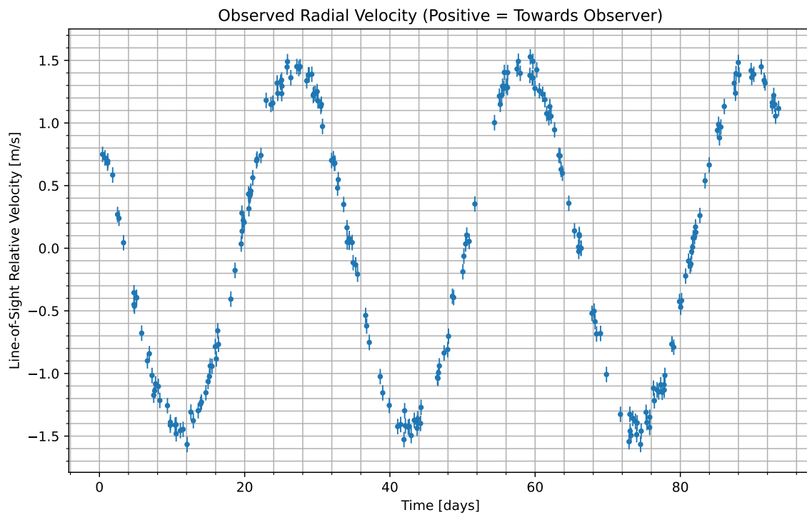
Figure 1: We have isolated the radial velocity of the host star due to the candidate planet. Data begins at UTC 2072-03-23/19:24. Positive values indicate the velocity at which the star is moving towards us; negative indicate the velocity at which it is moving away.
