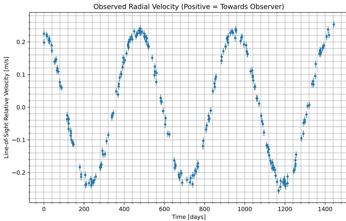
Figure 1: We have isolated the radial velocity of the host star due to the candidate planet. Data begins at UTC 2080-01-14/07:51. Positive values indicate the velocity at which the star is moving towards us; negative indicate the velocity at which it is moving away.
