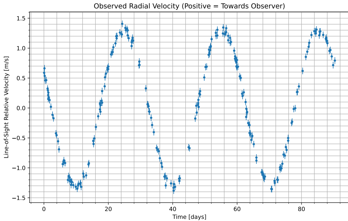
Figure 1: We have isolated the radial velocity of the host star due to the candidate planet. Data begins at UTC 2077-08-14/12:58. Positive values indicate the velocity at which the star is moving towards us; negative indicate the velocity at which it is moving away.
