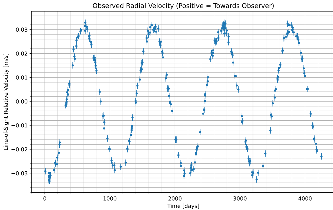
Figure 1: We have isolated the radial velocity of the host star due to the candidate planet. Data begins at UTC 2085-10-13/06:56. Positive values indicate the velocity at which the star is moving towards us; negative indicate the velocity at which it is moving away.
