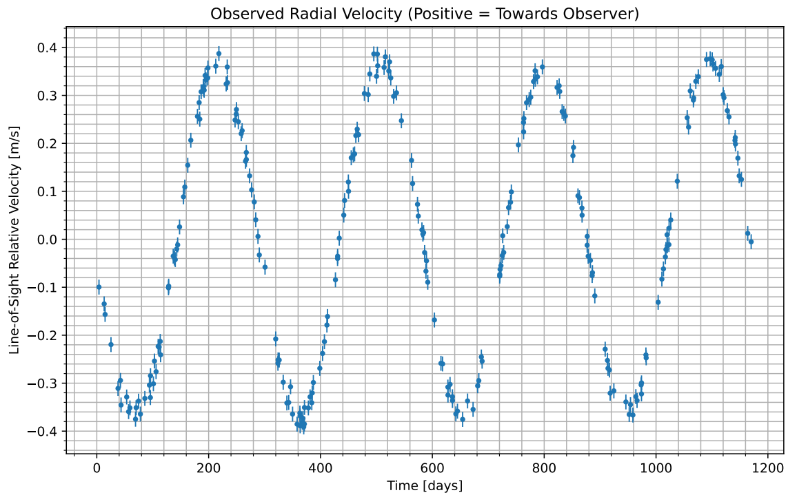
Figure 1: We have isolated the radial velocity of the host star due to the candidate planet. Data begins at UTC 2079-11-11/15:29. Positive values indicate the velocity at which the star is moving towards us; negative indicate the velocity at which it is moving away.
