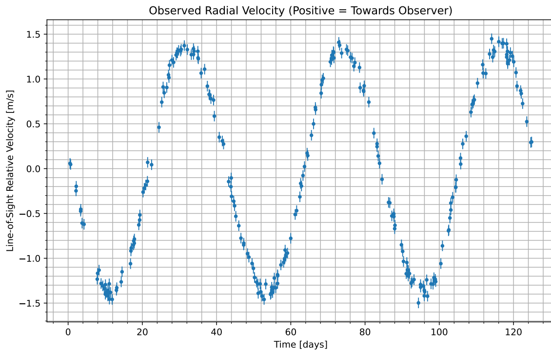
Figure 1: We have isolated the radial velocity of the host star due to the candidate planet. Data begins at UTC 2073-09-22/03:39. Positive values indicate the velocity at which the star is moving towards us; negative indicate the velocity at which it is moving away.
