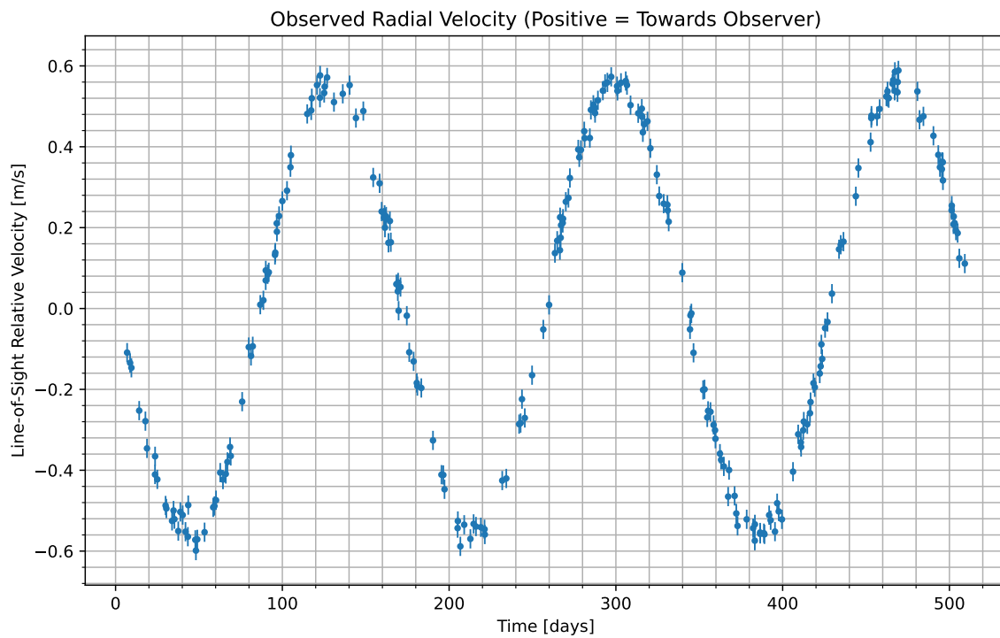
Figure 1: We have isolated the radial velocity of the host star due to the candidate planet. Data begins at UTC 2072-04-27/19:35. Positive values indicate the velocity at which the star is moving towards us; negative indicate the velocity at which it is moving away.
