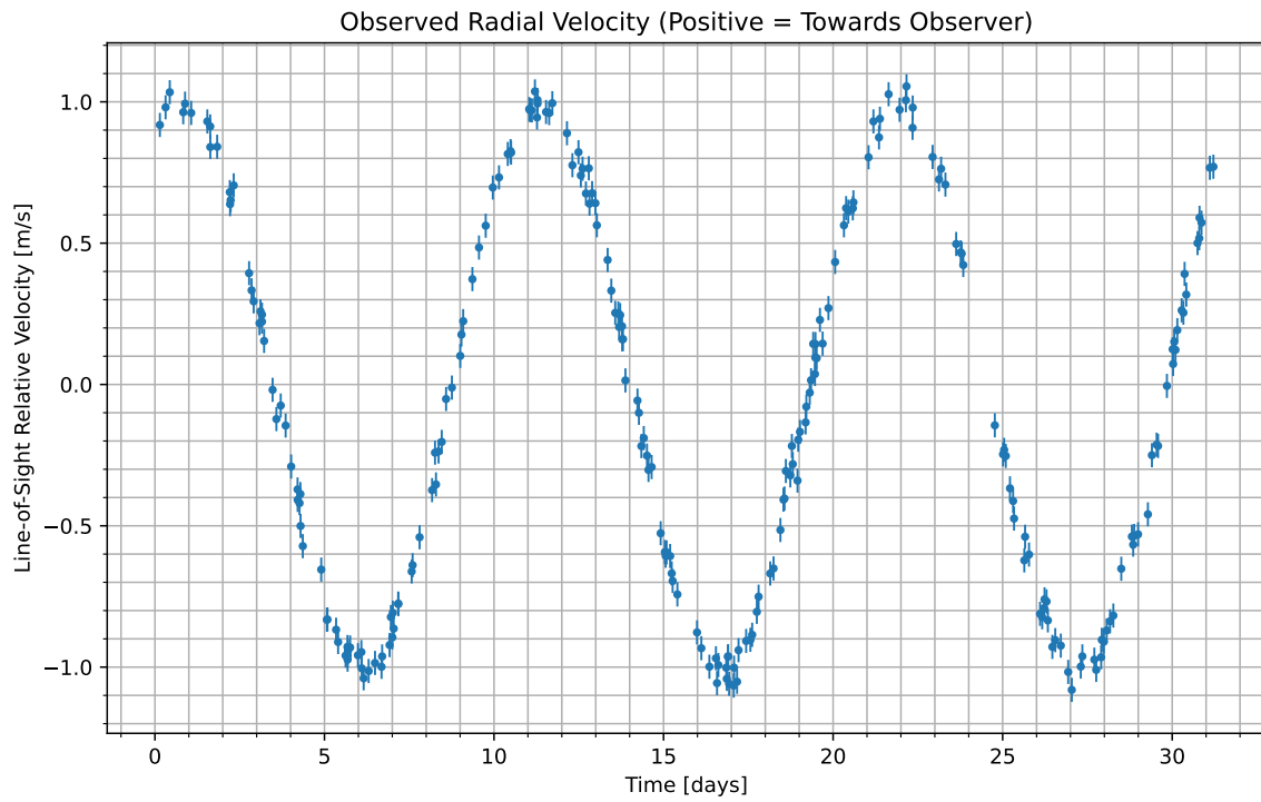
Figure 1: We have isolated the radial velocity of the host star due to the candidate planet. Data begins at UTC 2077-01-20/16:17. Positive values indicate the velocity at which the star is moving towards us; negative indicate the velocity at which it is moving away.
