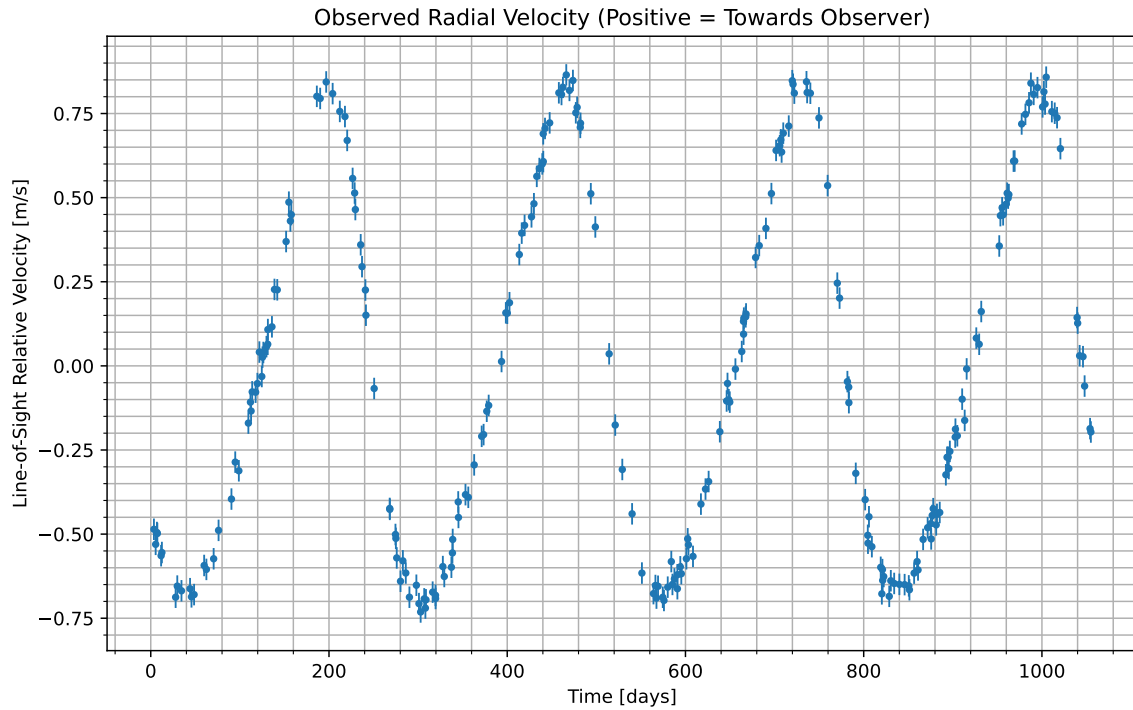
Figure 1: We have isolated the radial velocity of the host star due to the candidate planet. Data begins at UTC 2084-07-03/06:22. Positive values indicate the velocity at which the star is moving towards us; negative indicate the velocity at which it is moving away.
