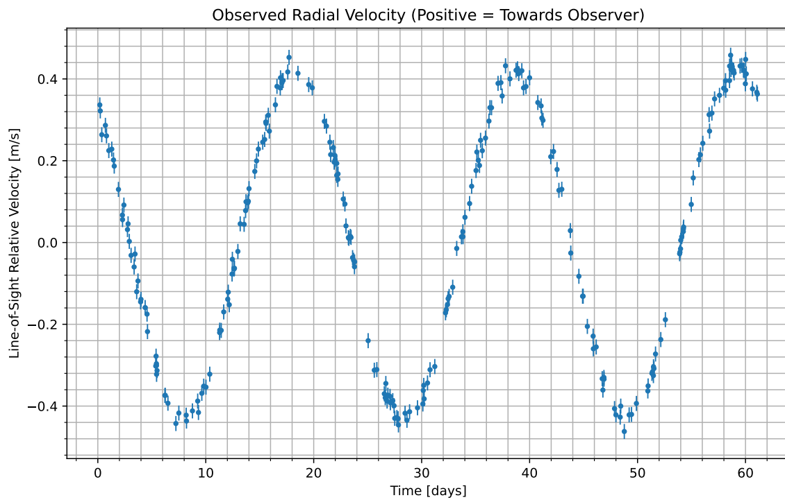
Figure 1: We have isolated the radial velocity of the host star due to the candidate planet. Data begins at UTC 2070-06-18/02:18. Positive values indicate the velocity at which the star is moving towards us; negative indicate the velocity at which it is moving away.
