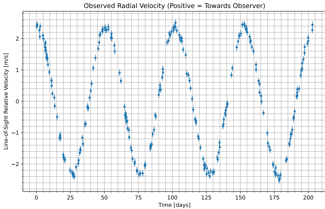
Figure 1: We have isolated the radial velocity of the host star due to the candidate planet. Data begins at UTC 2079-05-07/10:20. Positive values indicate the velocity at which the star is moving towards us; negative indicate the velocity at which it is moving away.
