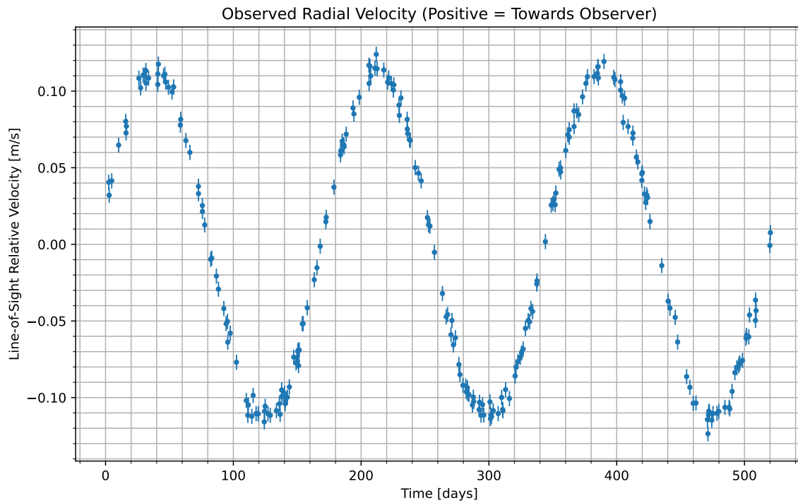
Figure 1: We have isolated the radial velocity of the host star due to the candidate planet. Data begins at UTC 2098-02-09/19:04. Positive values indicate the velocity at which the star is moving towards us; negative indicate the velocity at which it is moving away.
