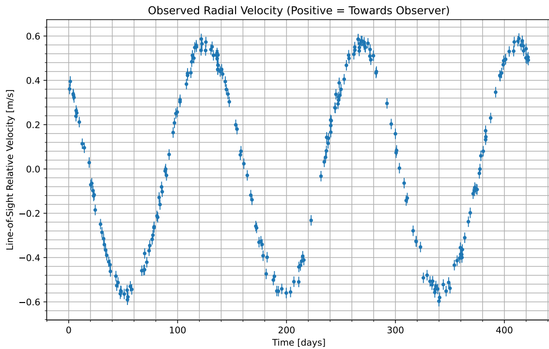
Figure 1: We have isolated the radial velocity of the host star due to the candidate planet. Data begins at UTC 2089-08-21/00:46. Positive values indicate the velocity at which the star is moving towards us; negative indicate the velocity at which it is moving away.
