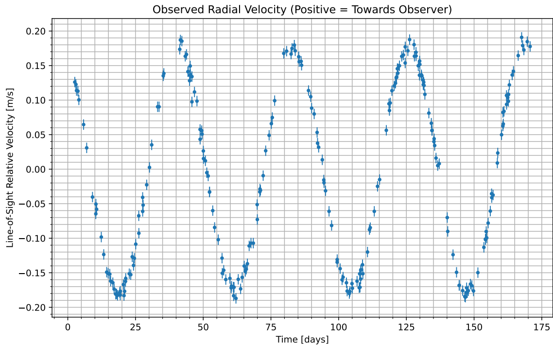
Figure 1: We have isolated the radial velocity of the host star due to the candidate planet. Data begins at UTC 2077-03-30/01:16. Positive values indicate the velocity at which the star is moving towards us; negative indicate the velocity at which it is moving away.
