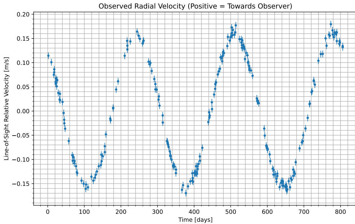
Figure 1: We have isolated the radial velocity of the host star due to the candidate planet. Data begins at UTC 2085-10-03/12:06. Positive values indicate the velocity at which the star is moving towards us; negative indicate the velocity at which it is moving away.
