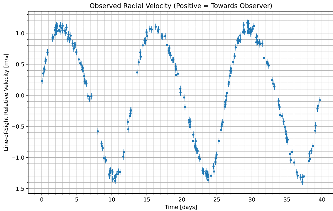
Figure 1: We have isolated the radial velocity of the host star due to the candidate planet. Data begins at UTC 2083-02-19/10:18. Positive values indicate the velocity at which the star is moving towards us; negative indicate the velocity at which it is moving away.
