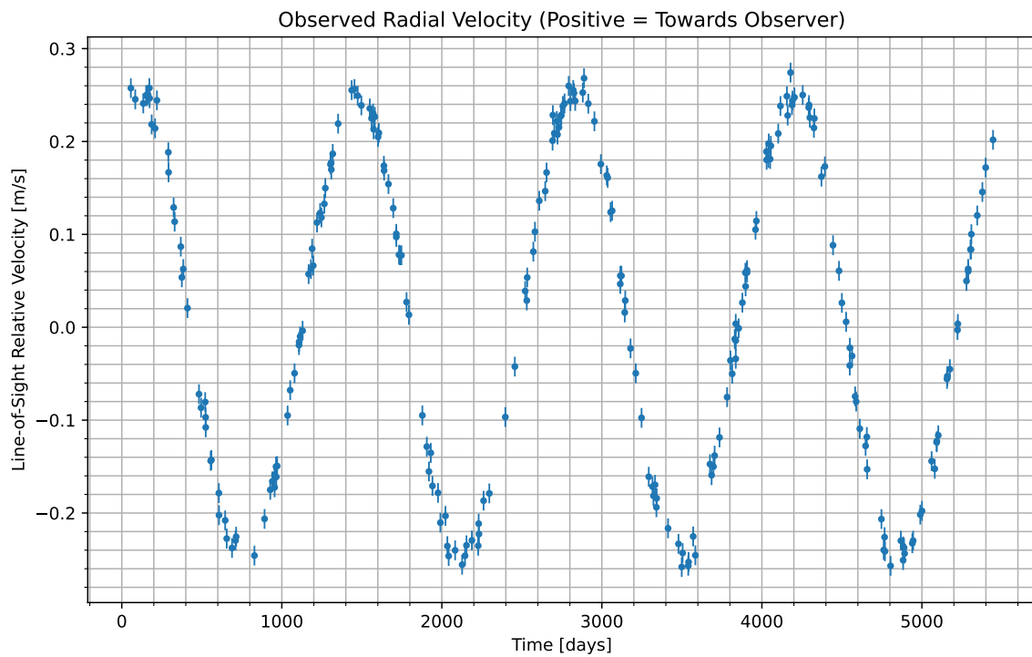
Figure 1: We have isolated the radial velocity of the host star due to the candidate planet. Data begins at UTC 2081-06-06/22:32. Positive values indicate the velocity at which the star is moving towards us; negative indicate the velocity at which it is moving away.
