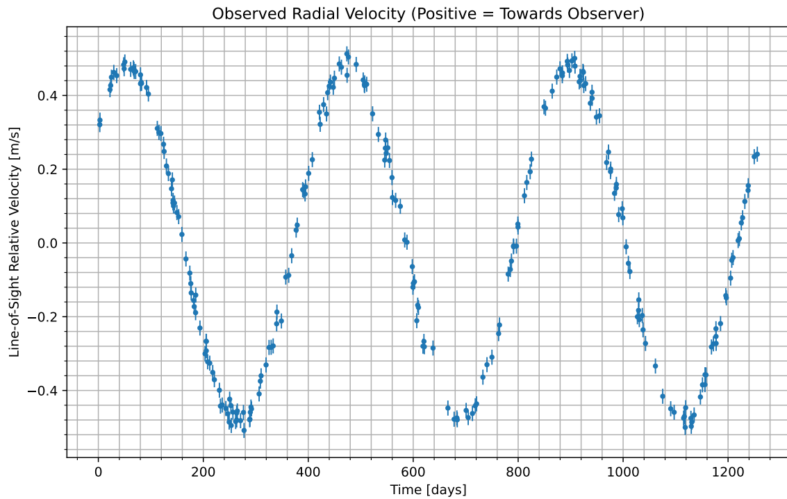
Figure 1: We have isolated the radial velocity of the host star due to the candidate planet. Data begins at UTC 2077-05-04/19:44. Positive values indicate the velocity at which the star is moving towards us; negative indicate the velocity at which it is moving away.
