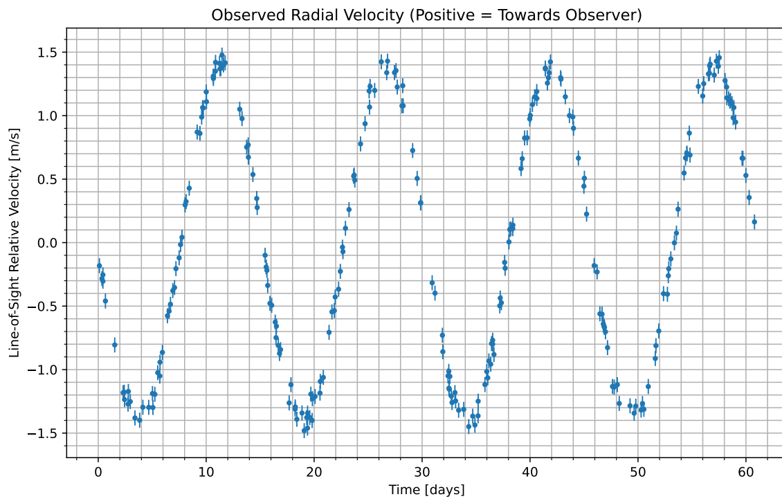
Figure 1: We have isolated the radial velocity of the host star due to the candidate planet. Data begins at UTC 2099-12-27/17:01. Positive values indicate the velocity at which the star is moving towards us; negative indicate the velocity at which it is moving away.
