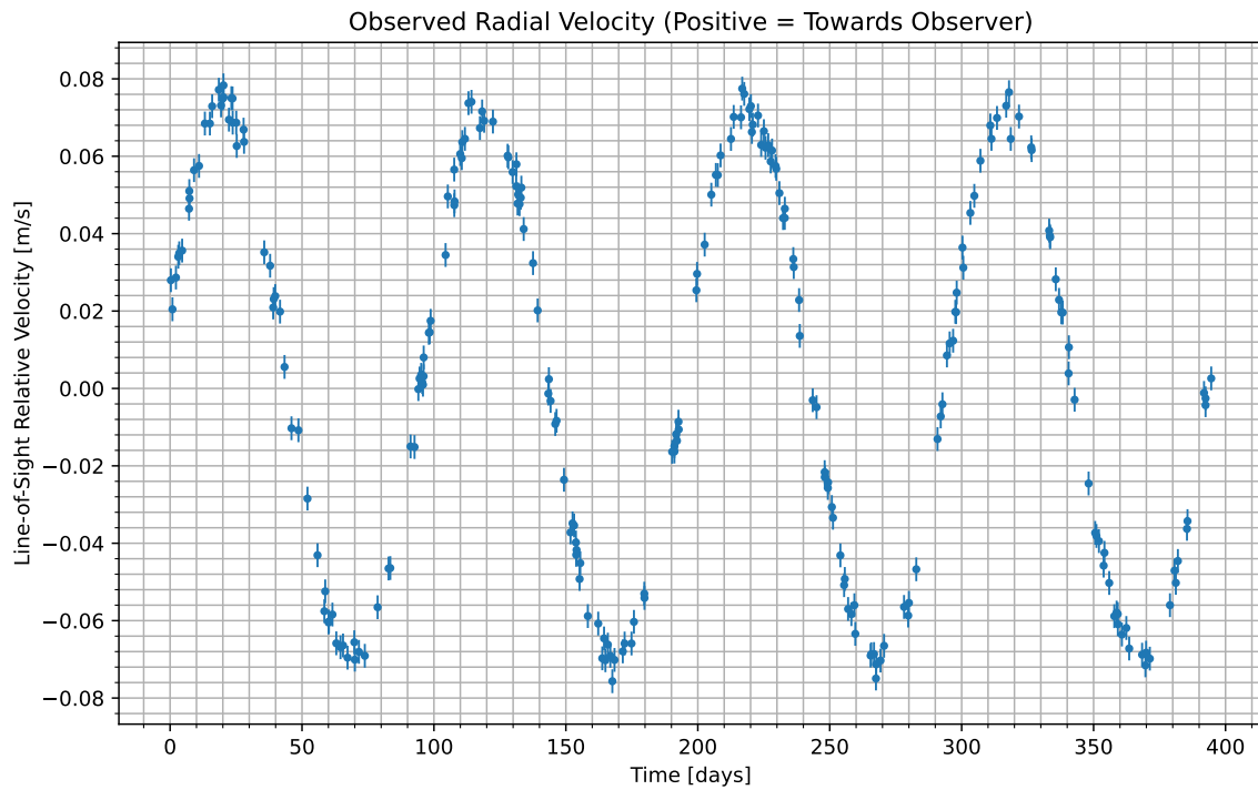
Figure 1: We have isolated the radial velocity of the host star due to the candidate planet. Data begins at UTC 2085-08-09/12:39. Positive values indicate the velocity at which the star is moving towards us; negative indicate the velocity at which it is moving away.
