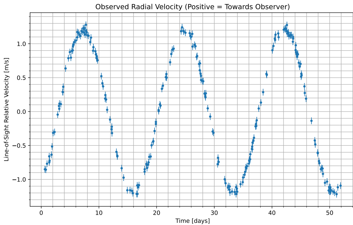
Figure 1: We have isolated the radial velocity of the host star due to the candidate planet. Data begins at UTC 2074-11-11/09:39. Positive values indicate the velocity at which the star is moving towards us; negative indicate the velocity at which it is moving away.
