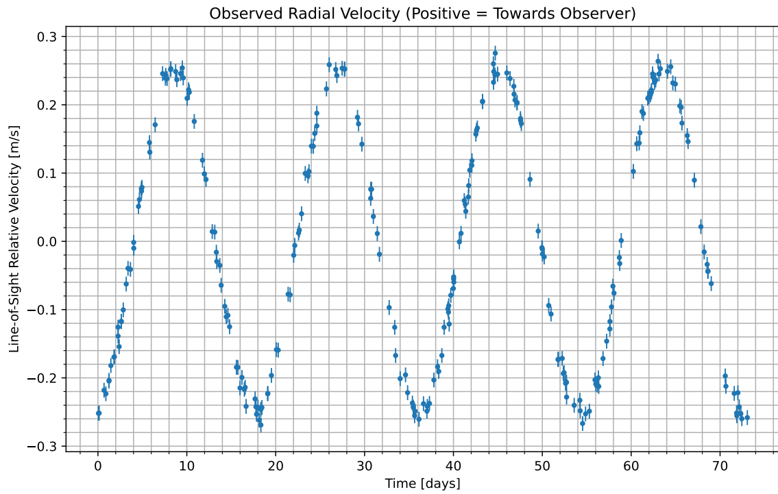
Figure 1: We have isolated the radial velocity of the host star due to the candidate planet. Data begins at UTC 2078-12-16/07:37. Positive values indicate the velocity at which the star is moving towards us; negative indicate the velocity at which it is moving away.
