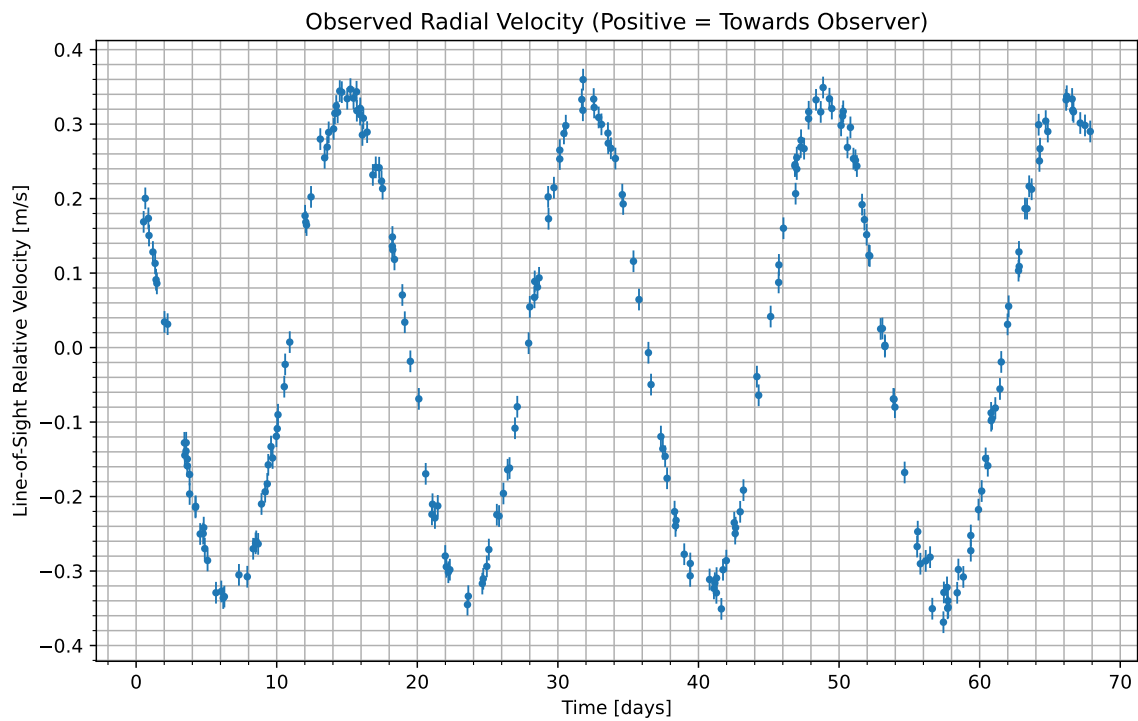
Figure 1: We have isolated the radial velocity of the host star due to the candidate planet. Data begins at UTC 2080-10-24/09:34. Positive values indicate the velocity at which the star is moving towards us; negative indicate the velocity at which it is moving away.
