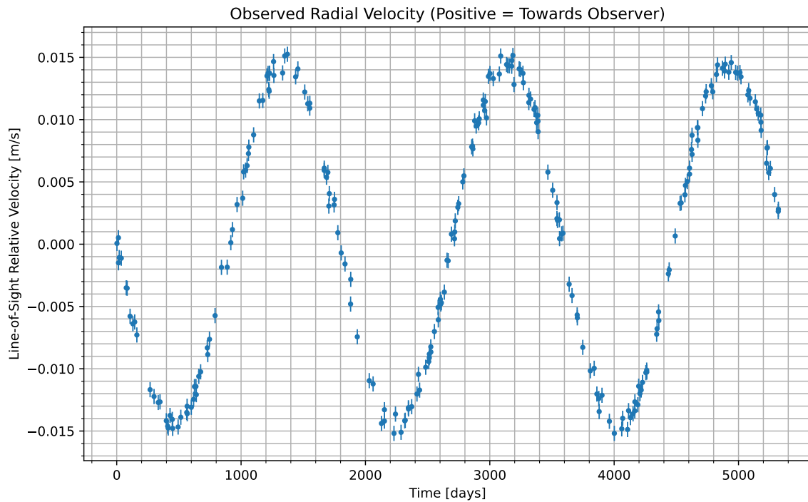
Figure 1: We have isolated the radial velocity of the host star due to the candidate planet. Data begins at UTC 2067-04-15/04:10. Positive values indicate the velocity at which the star is moving towards us; negative indicate the velocity at which it is moving away.
