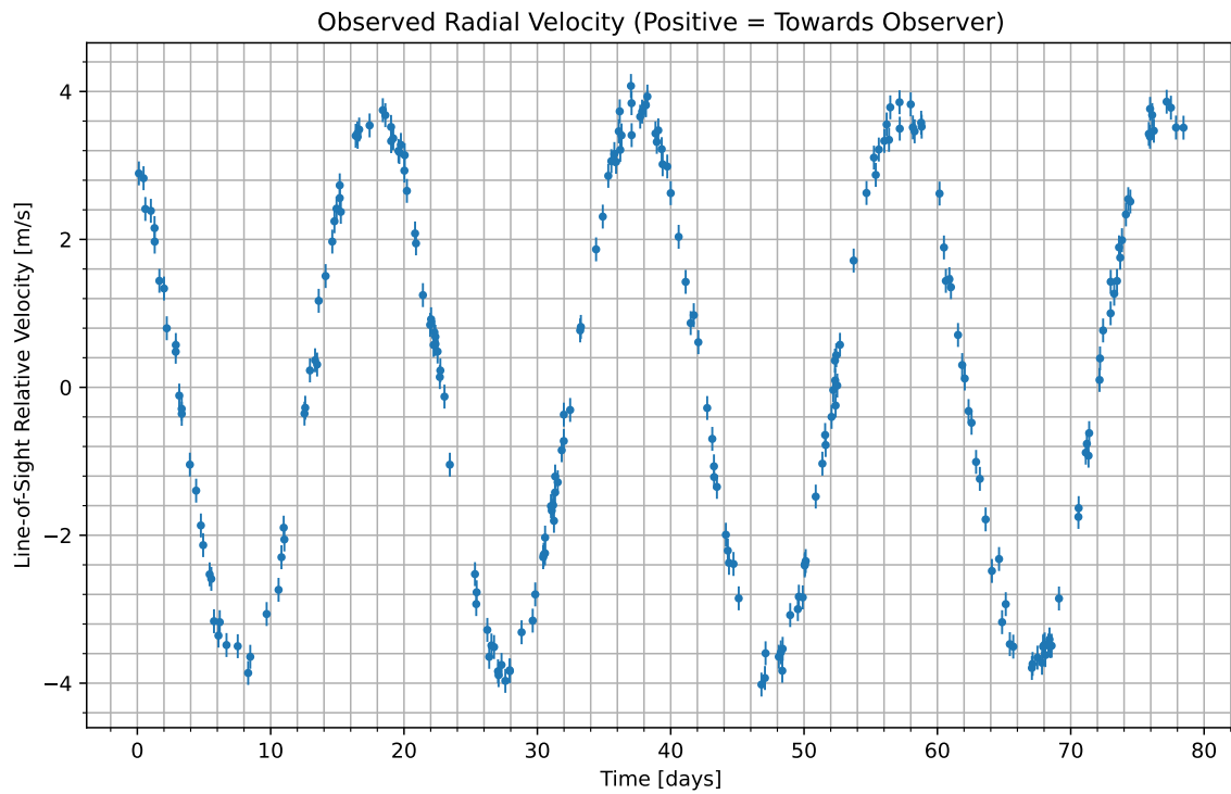
Figure 1: We have isolated the radial velocity of the host star due to the candidate planet. Data begins at UTC 2081-01-08/01:19. Positive values indicate the velocity at which the star is moving towards us; negative indicate the velocity at which it is moving away.
