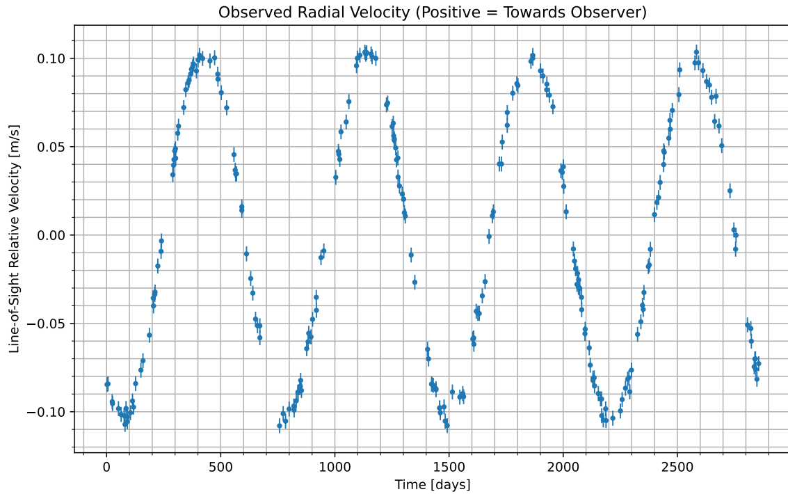
Figure 1: We have isolated the radial velocity of the host star due to the candidate planet. Data begins at UTC 2063-07-04/19:18. Positive values indicate the velocity at which the star is moving towards us; negative indicate the velocity at which it is moving away.
