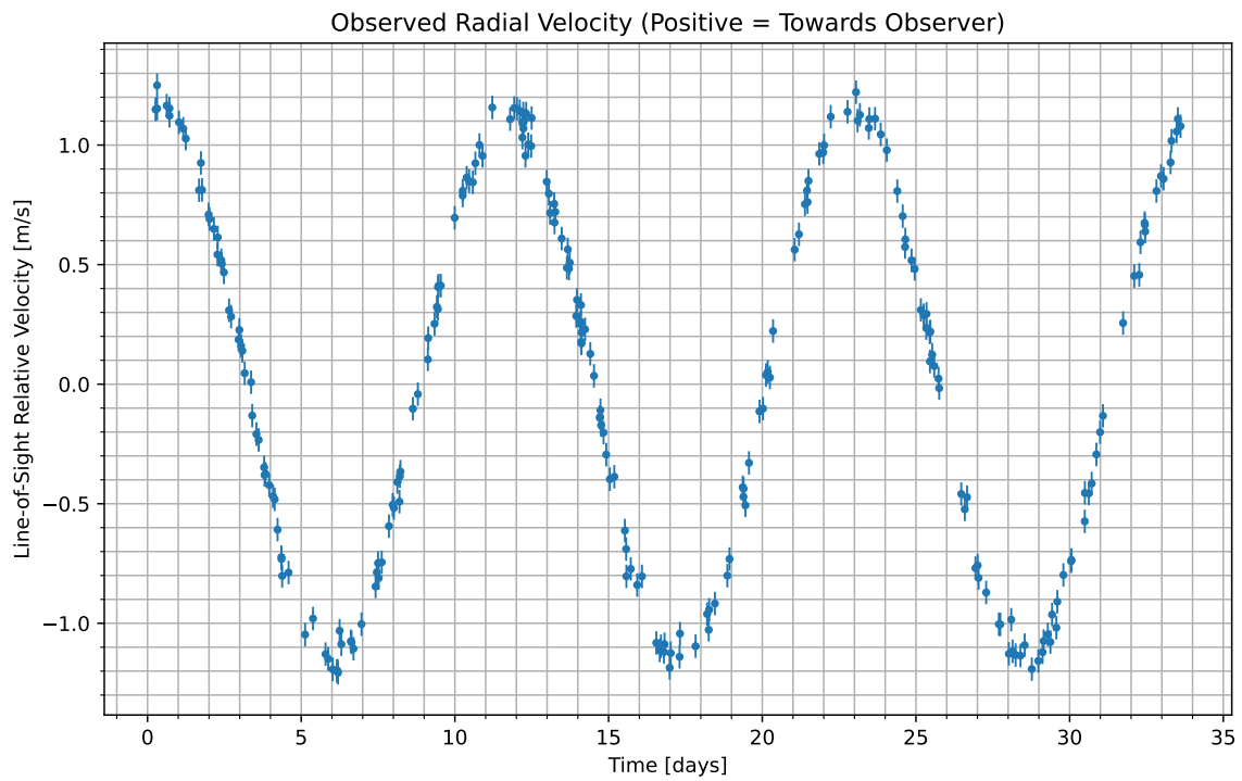
Figure 1: We have isolated the radial velocity of the host star due to the candidate planet. Data begins at UTC 2086-12-26/20:18. Positive values indicate the velocity at which the star is moving towards us; negative indicate the velocity at which it is moving away.
