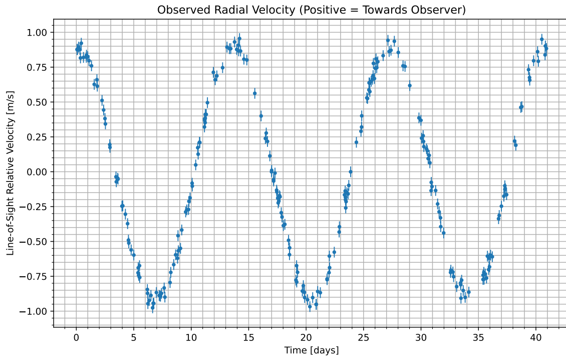
Figure 1: We have isolated the radial velocity of the host star due to the candidate planet. Data begins at UTC 2082-06-26/12:02. Positive values indicate the velocity at which the star is moving towards us; negative indicate the velocity at which it is moving away.
