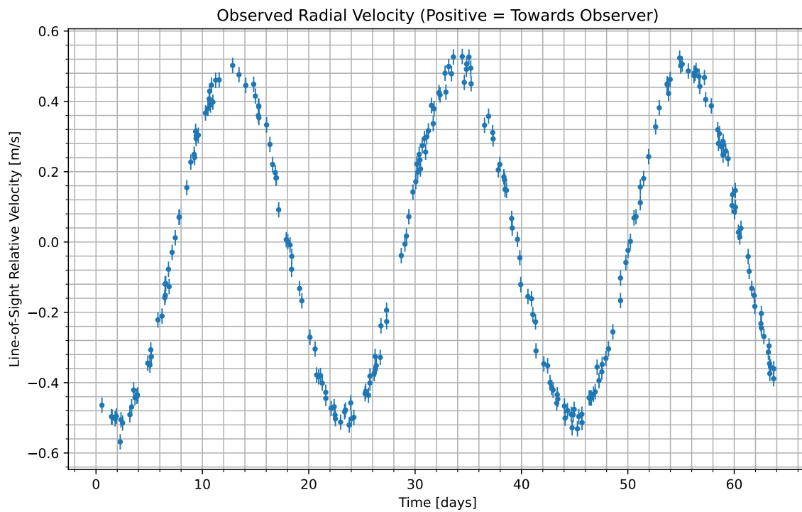
Figure 1: We have isolated the radial velocity of the host star due to the candidate planet. Data begins at UTC 2085-09-21/07:51. Positive values indicate the velocity at which the star is moving towards us; negative indicate the velocity at which it is moving away.
