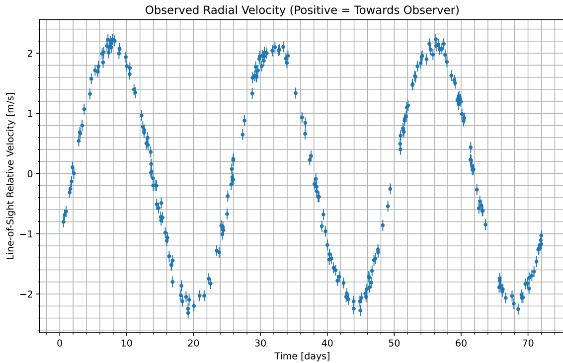
Figure 1: We have isolated the radial velocity of the host star due to the candidate planet. Data begins at UTC 2078-10-18/06:58. Positive values indicate the velocity at which the star is moving towards us; negative indicate the velocity at which it is moving away.
