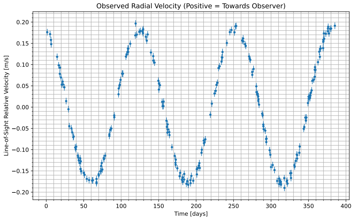
Figure 1: We have isolated the radial velocity of the host star due to the candidate planet. Data begins at UTC 2087-07-08/16:53. Positive values indicate the velocity at which the star is moving towards us; negative indicate the velocity at which it is moving away.
