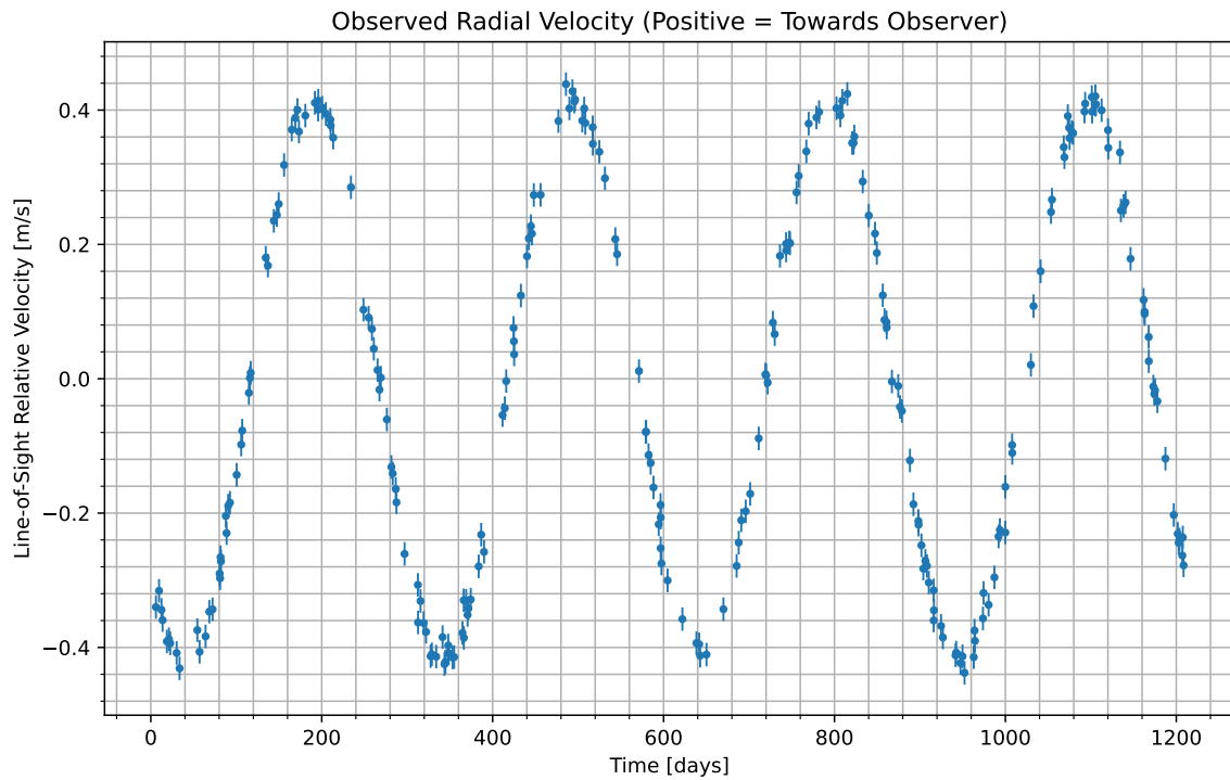
Figure 1: We have isolated the radial velocity of the host star due to the candidate planet. Data begins at UTC 2066-09-07/18:05. Positive values indicate the velocity at which the star is moving towards us; negative indicate the velocity at which it is moving away.
