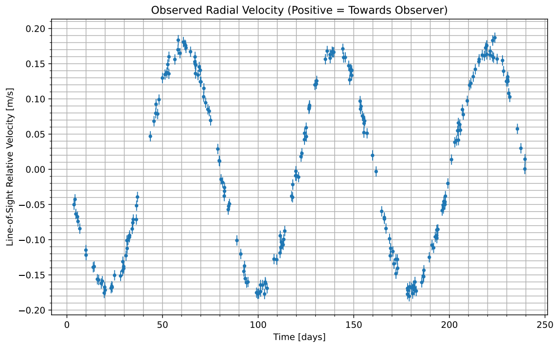
Figure 1: We have isolated the radial velocity of the host star due to the candidate planet. Data begins at UTC 2080-11-18/21:56. Positive values indicate the velocity at which the star is moving towards us; negative indicate the velocity at which it is moving away.
