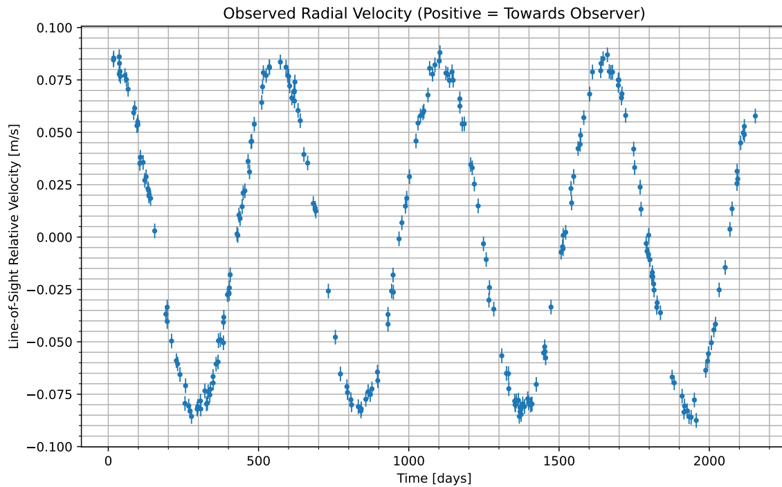
Figure 1: We have isolated the radial velocity of the host star due to the candidate planet. Data begins at UTC 2091-12-11/16:24. Positive values indicate the velocity at which the star is moving towards us; negative indicate the velocity at which it is moving away.
