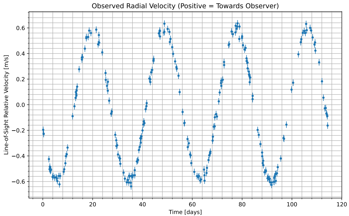
Figure 1: We have isolated the radial velocity of the host star due to the candidate planet. Data begins at UTC 2094-03-16/03:17. Positive values indicate the velocity at which the star is moving towards us; negative indicate the velocity at which it is moving away.
