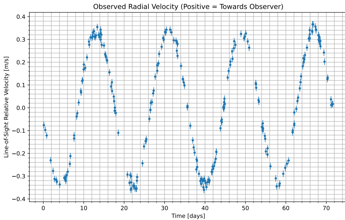
Figure 1: We have isolated the radial velocity of the host star due to the candidate planet. Data begins at UTC 2095-02-24/23:38. Positive values indicate the velocity at which the star is moving towards us; negative indicate the velocity at which it is moving away.
